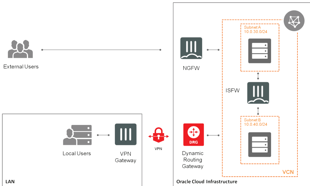
FortiGate-VM on OCI deployment as NGFW, ISFW and VPN Gateway
