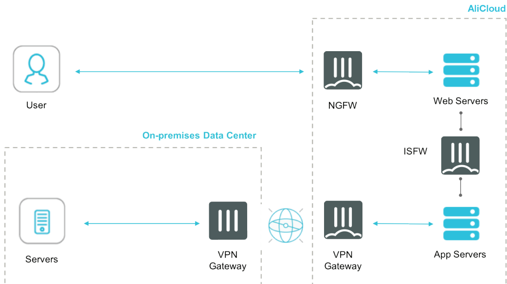
FortiGate-VM on AliCloud deployment as NGFW, ISFW and VPN Gateway
