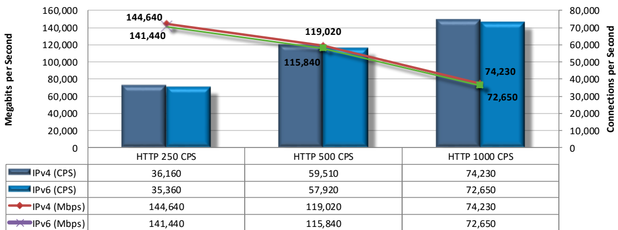
Figure 13 – HTTP Capacity with HTTP Persistent Connections
