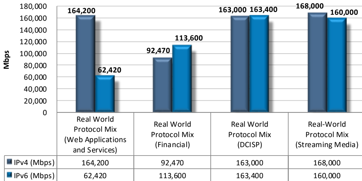
Figure 14 – “Real-World” Traffic Mixes
