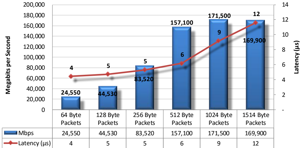
Figure 7 – Raw Packet Processing Performance – UDP Traffic (IPv4)
