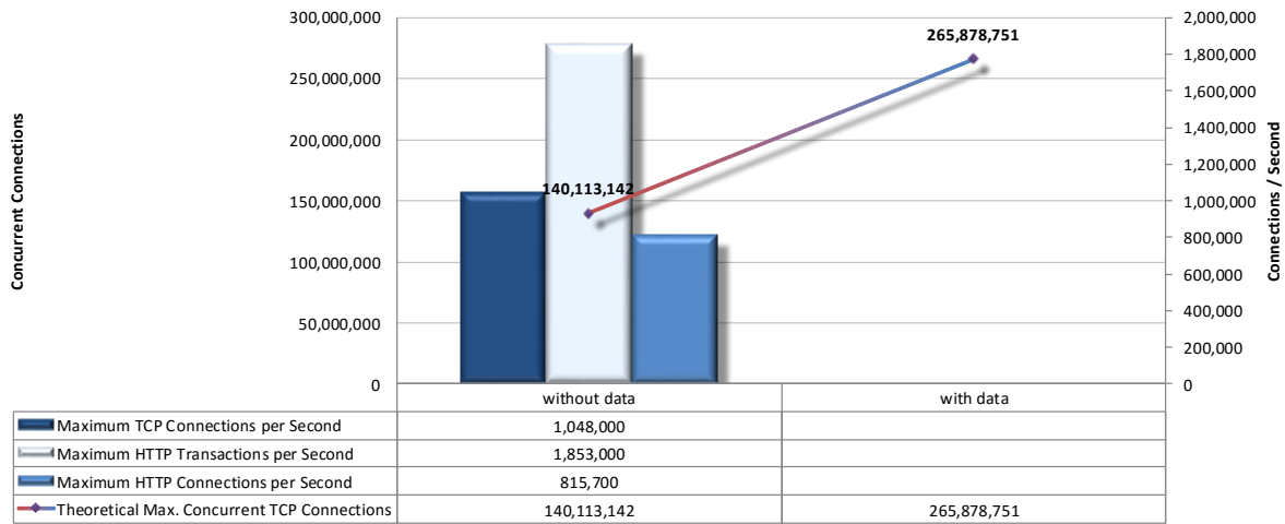
Figure 10 – Concurrency and Connection Rates (IPv6)
