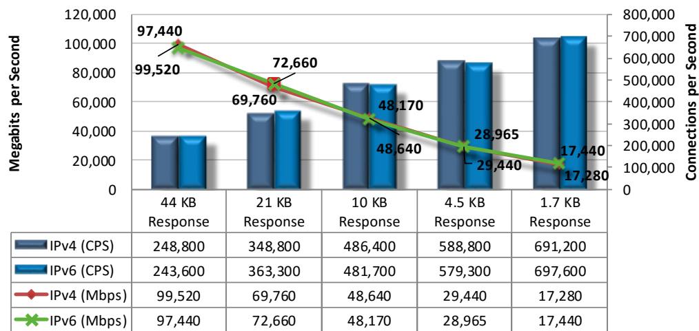
Figure 11 – HTTP Capacity with No Transaction Delays
